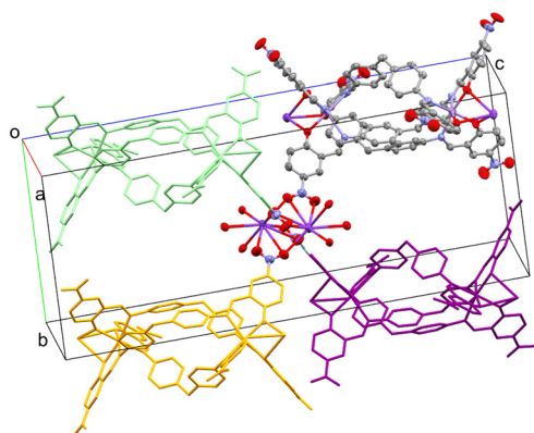
Fig. 4 Perspective view of the three-dimensional growth of 1 , promoted by the NO_2 groups and K^+ . The dinuclear K unit is drawn with ellipsoids at 30% probability level. The coordinated NO_2 to the K dinuclear node come from different helicate units, highlighted in different colors and in a capped stick style. Solvent molecules and H-atoms are omitted for the sake of clarity.
