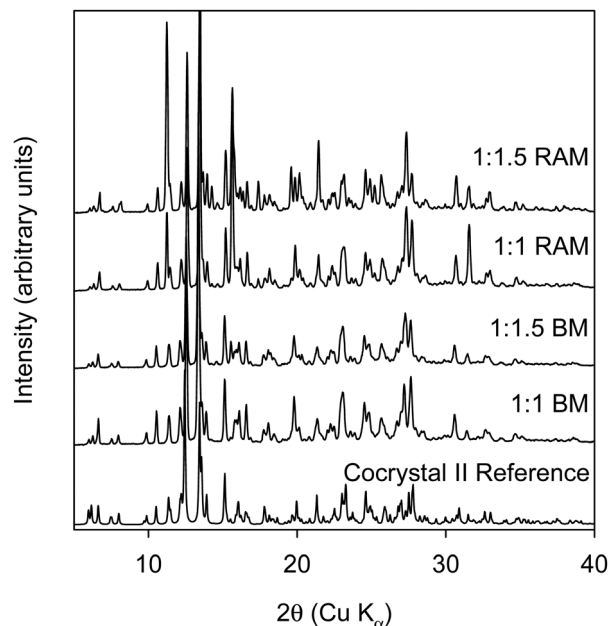
Fig. 5 XRPD data of rBN/BQ subjected to RAM shown in comparison to the reference powder data calculated from the published crystal structure of cocrystal II. BM was performed at 25 Hz for 10 minutes. RAM was performed at 75g for 90 minutes. Heptane was used as a liquid additive at an \eta of 0.5 for all experiments. 490–540 mg of total solids was used for all experiments.
