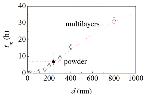
Fig. 4 The ignition time, t_{\text{ig}} , of multilayers (O) as a function of the bi-layer thickness, d . The vertical and horizontal dotted lines identify the ignition time of multilayers with d equal to 240 nm. The ignition time of the pristine Al–Ni powder mixture (●) is also shown. The dotted curve is a guide to the eyes.
