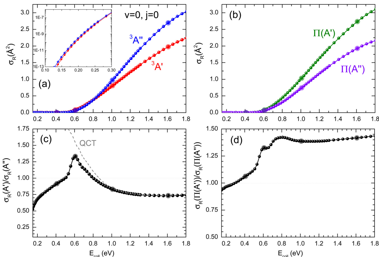
Fig. 1 (a) QM excitation function summed over final states for the \text{O}(^3\text{P}) + \text{D}_2 ( v=0, j=0 ) reaction on the ^3A' (red) and ^3A'' PES (blue). The inset represents the excitation function for low E_{\text{coll}} in the logarithm scale. (b) QM excitation function resolved in the two \Lambda -doublet manifolds: \Pi(A') (dark green) and \Pi(A'') (purple). (c) Ratio between the QM cross sections on the ^3A' and ^3A'' PES as a function of E_{\text{coll}} . QCT results are shown as the dashed grey lines. (d) Ratio between the QM cross sections resolved in the two \Lambda -doublet manifolds. Results for E_{\text{coll}} = 0.41 \text{ eV} , 0.6 \text{ eV} , 1.0 \text{ eV} , and 1.6 \text{ eV} , for which P(J) and DCS are shown in Fig. 2 and/or Fig. 3 and 4 are highlighted.
