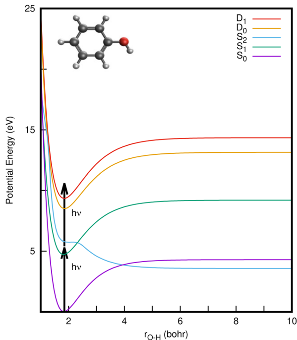
Fig. 1 One-dimensional cuts of the (diabatic) potential energy surfaces of phenol from the vibronic coupling model along the O–H stretching mode ( r_{\text{O-H}} ) for the S_0 ( 1^1\pi\pi^* ) ground state, and first two singlet excited states, S_1 ( 1^1\pi\pi^* ) and S_2 ( 1^1\pi\pi^* ). Potential energy cuts of the first two doublet states D_0 and D_1 of the phenol cation are also shown. The S_2/S_1 and S_2/S_0 states cross each other at 2.3 bohr and 3.95 bohr, respectively. 1+1 photon excitation from S_0 to D_0 and D_1 states, via the bright S_1 state is illustrated by vertical arrows. The inset depicts a schematic representation of the optimized geometry of phenol in the ground state.
