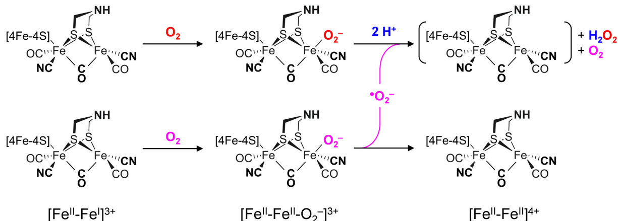
Scheme 1 Binding and reduction of \text{O}_2 at the H-cluster in the [\text{Fe}^{\text{II}}-\text{Fe}] state ( \text{H}_{\text{ox}} ) produces the [\text{Fe}^{\text{II}}-\text{Fe}^{\text{II}}-\text{O}_2^-] state ( \text{H}_{\text{ox}}-\text{O}_2 ) stabilized by hydrogen bonding between ligands adt and \text{O}_2^- (dashed lines). Protonation and disproportionation of superoxide leads to \text{H}_2\text{O}_2 formation and regeneration of \text{O}_2 . We presume that the [\text{Fe}^{\text{II}}-\text{Fe}^{\text{II}}] state is unstable and will continue decaying.
