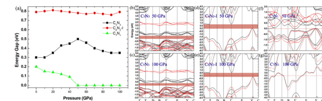
Fig. 11 (a) The pressure-dependent energy gap of C_5N_3 , C_6N_2-I , and C_7N_1 systems. (b)–(g) The band structures for the three systems under 50 and 100 GPa external pressures, respectively. The black and red lines in the band structures represent the results obtained from the PBE and HSE functionals, respectively.
