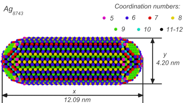
Fig. 4 Coordination numbers, longitudinal and transverse plasmon length for an Ag nanorod containing 8743 atoms. From ref. 75.
