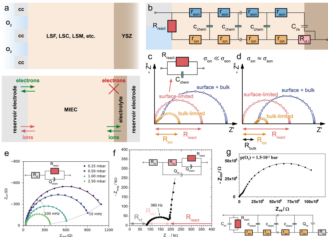
Fig. 6 (a) Sketch (top) and schematic representation (bottom) of a dense SOFC electrode consisting of an MIEC on a YSZ electrolyte, with a current collector (cc) contacting the MIEC on the O_2 -exposed side. (b) Adapted transmission line for the SOFC electrode in subfigure (a). (c) Calculated impedance response of the SOFC electrode with a predominant electronic conductor (LSF, \sigma_{ion} \ll \sigma_{eon} ) for different limiting cases. (d) Calculated impedance response of the SOFC electrode with a mixed conductor (STF at low pO_2 , \sigma_{ion} \approx \sigma_{eon} ) for different limiting cases. (e) pO_2 -dependent half-cell impedance spectra of an LSF thin film grown on top of a Pt-grid current collector on a YSZ single crystal. Original image published in ref. 8 under a CC BY license. (f) Impedance response of an LSCF thin film microelectrode on a YSZ single crystal. Image reprinted (adapted) from ref. 49 with permission from Elsevier. (g) Impedance response of an LSM thin film microelectrode on a YSZ single crystal. Image reprinted (adapted) from ref. 50 with permission from John Wiley and Sons. For subfigures (e)–(g), the equivalent circuits used for impedance fits were added to the image.
