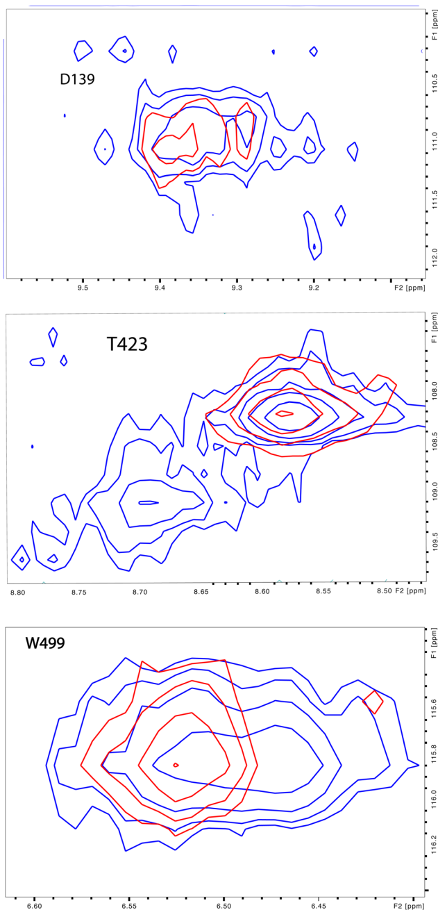
Fig. 6 Preferential population of CYP17A1/abiraterone major conformation upon binding of cytb 5 . ^1\text{H} - ^{15}\text{N} correlations for Asp 139 (C-D loop), Thr 423 ( \beta -meander) and Trp 499 ( \beta 5 strand) in the absence (blue) and presence (red) of 0.4 equivalents of cytb 5 .
