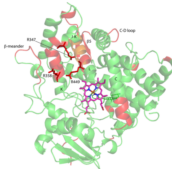
Fig. 7 Distribution of regions (in red) showing conformational selection in CYP17A1/abiraterone upon binding of cytb 5 . The view is of the proximal surface, rotated \sim 60^\circ counterclockwise from Fig. 3. Regions shown in orange are tentative, either due to spectral overlap or provisional resonance assignment. The side chains of arginine residues (R347, R358 and R449) implicated in cytb 5 binding are shown in red.
