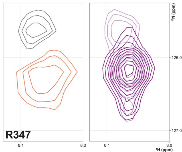
Fig. 8 (right) Overlay of ^1\text{H} - ^{15}\text{N} correlation for Arg 347 in the absence (light contours) and presence (dark contours) of 0.4 equivalents of cytb 5 . (left) Spectral subtraction of the same correlation with black contours representing loss of signal and orange showing increased intensity upon addition of cytb 5 .
