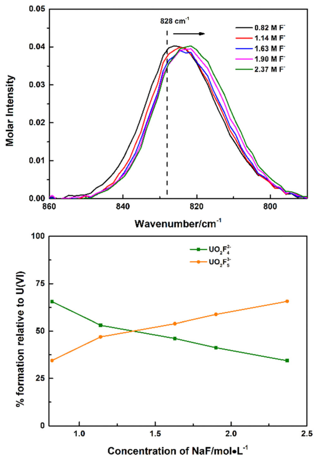
Fig. 2 Raman spectra of \text{UO}_2(\text{NO}_3)_2 in 2.5 M (\text{CH}_3)_4\text{NNO}_3/(\text{CH}_3)_4\text{NNO}_3 (top) and speciation distribution during titration (bottom). C_{\text{Uranium}} = 0.059 M, C_{\text{nitrate}} = 0.118\text{--}1.69 M, V = 1.0 mL, C_{\text{H}^+} = 0.002 M, C_{\text{fluoride}} = 0.82\text{--}2.37 M.
