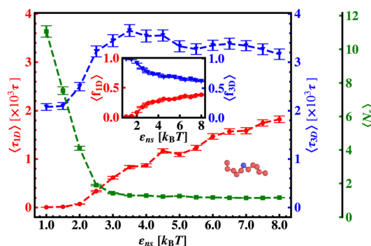
Fig. 10 The average one dimensional search time per search round, \langle \tau_{1D} \rangle , (red '—●—' line), the average three dimensional search time per search round, \langle \tau_{3D} \rangle , (blue '—▼—' line), and the corresponding average number of search rounds, \langle N_s \rangle (green '—■—' dashed line) as a function of non-specific interaction strength, \epsilon_{ns} , when the target is at the center of a flexible DNA. The inset figure shows the variation of the average of the fractions of one dimensional search time, \langle f_{1D} \rangle = \langle \tau_{1D} / (\tau_{1D} + \tau_{3D}) \rangle (red '—●—' line) and three dimensional search time, \langle f_{3D} \rangle = \langle \tau_{3D} / (\tau_{1D} + \tau_{3D}) \rangle (blue '—▼—' line) with non-specific interaction strength, \epsilon_{ns} , when the target is placed at the center of a flexible DNA.
