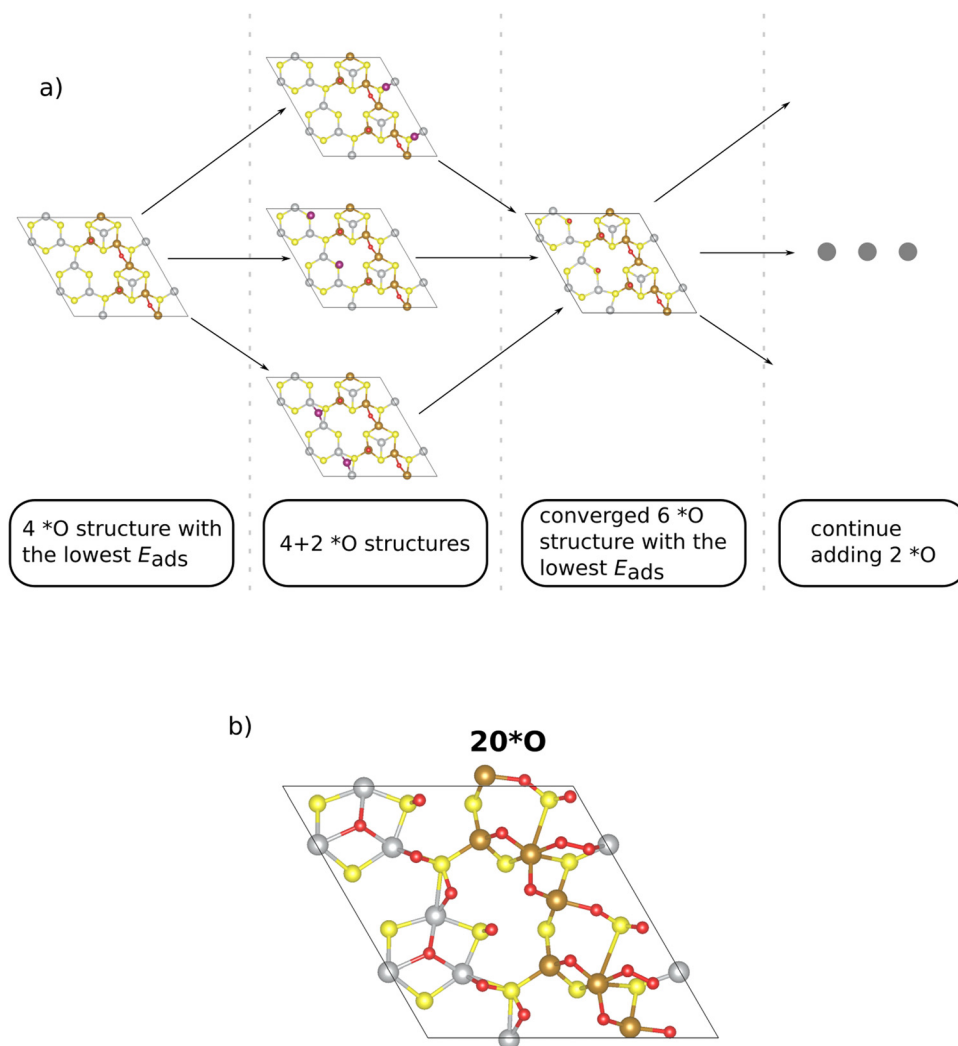
Fig. 2 (a) Visualization of the iterative procedure to determine the surface structure of oxygen coverages on the Pn(111) surface. (b) A coverage of 20^*O is identified as the active phase under typical OER conditions ( U = 1.53 V vs. RHE), and we make use of this phase to discuss the active site, limiting step, and the contribution of solvation.
