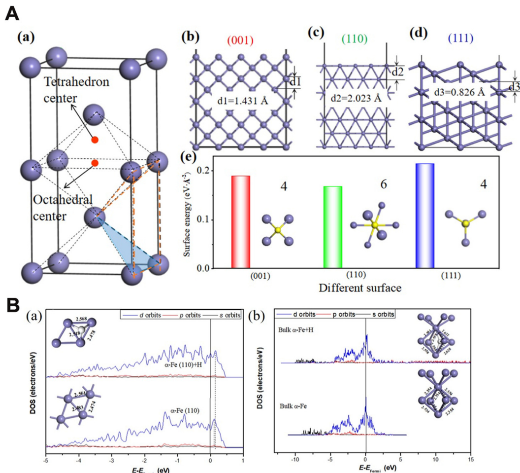
Fig. 5 (A) The coordination of atoms along different crystallographic orientations are shown in the figure. (a) geometry of (1 \times 1 \times 2) \alpha -Fe surfaces. (b) \alpha -Fe(001). (c) \alpha -Fe(110). (d) \alpha -Fe(111). (e) Calculated surface energies for the above surfaces. The adsorption, absorption and diffusion of H atoms are intimately connected to the nearest neighbour atoms and coordination number of the planes. Reproduced from ref. 36 with permission from Elsevier, copyright 2023. (B) The density of states (DOS) calculated for bulk and Fe surface and the changes in electronic structure brought by the presence of H. (a) and (b) represent calculated partial density of states of Fe on \alpha -Fe(110) and that of H adsorbed on bulk \alpha -Fe respectively. The DOS can serve as a valuable tool to provide information about the changes in orbital hybridization brought by the presence of H in the crystal lattice and the bonding characteristics. Reproduced from ref. 36 with permission from Elsevier, copyright 2023.
