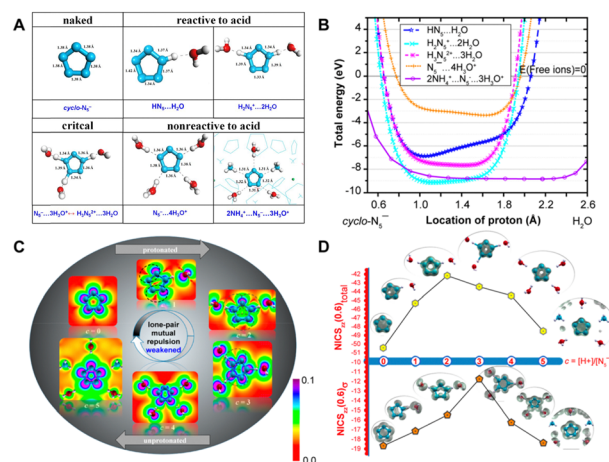
Fig. 4 (A) Optimized structures of the cyclo -N 5 - complex/crystal at various acid concentrations; (B) energetic landscape of the cyclo -N 5 - complex/crystal as a function of the N–H distance; (C) LDOS at the antibonding energy level plotted in the equatorial plane of cyclo -N 5 - under varying acidities; (D) NICS zz (0.6) total and NICS zz (0.6) σ of the cyclo -N 5 - anion under varying acidities and the corresponding LDOS isosurfaces plotted for the lowest energy level (nonbonding) of the aromatic π- and σ-systems. Reproduced with permission from ref. 90. Copyright 2019, American Chemical Society.
