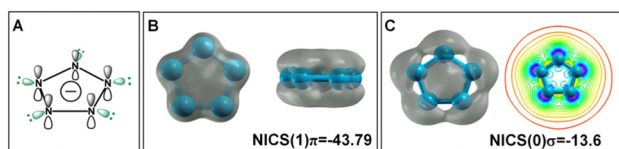
Fig. 3 (A) Atomic orbital diagram of the cyclo -N 5 - anion; (B) top and side views of the LDOS isosurface at the lowest energy level of the aromatic π-system; (C) LDOS isosurface at the lowest energy level of the aromatic σ-system. Reproduced with permission from ref. 91. Copyright 2019, Wiley.
