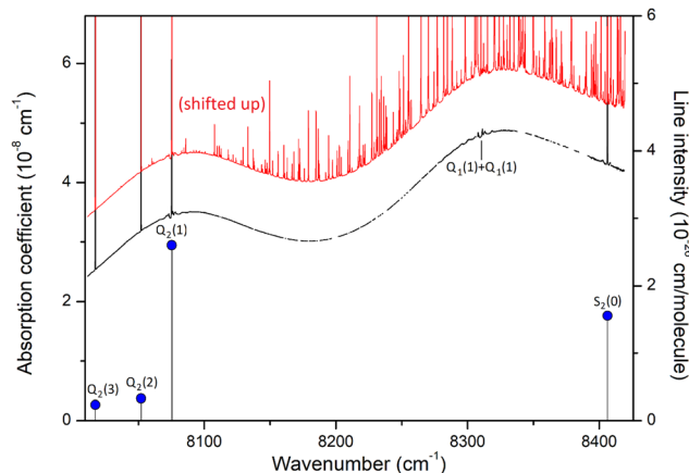
Fig. 2 Overview of the hydrogen spectrum at room temperature ( P = 760 Torr) in the 8000–8450 \text{cm}^{-1} interval of the first overtone band. The zero-absorption baseline due to the mirror reflectivity has been subtracted. The black curve is obtained after subtraction of the absorption lines of water vapor, visible on the red curve which has been shifted up by 10^{-8}\text{ cm}^{-1} for clarity. The mole fraction of water was about 25 ppm for this recording. The blue dots show the positions and intensities of the Q_2(1-3) and S_2(0) monomer lines. The calculated position of the Q_1(1) + Q_1(1) transition which is not radiatively allowed, is also indicated.
