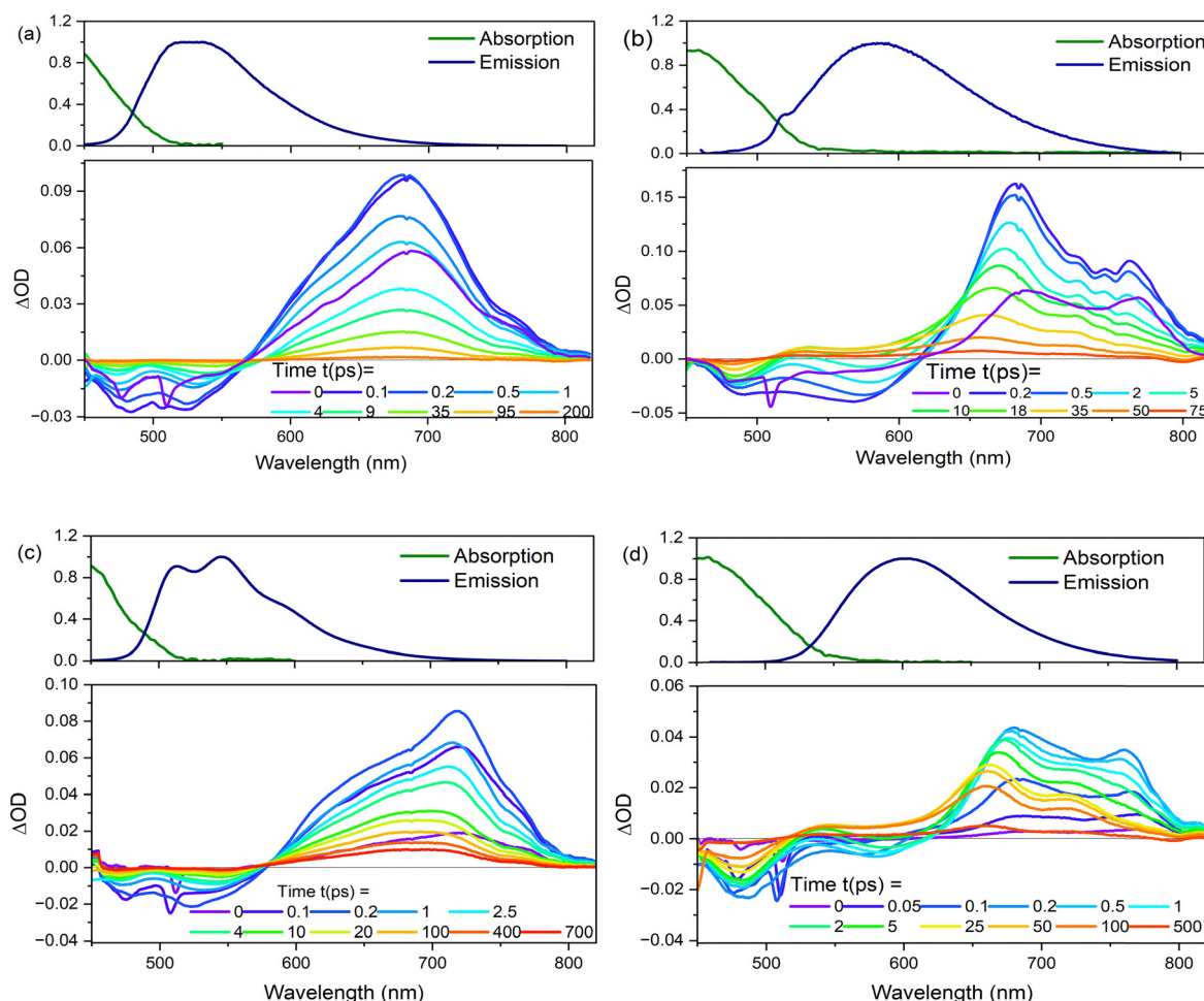
Fig. 8 Transient absorption spectra plotted as a function of different delays after the pump pulse for (a) 2 and (b) 3 in EtOH, and (c) 2 , and (d) 3 in THF at T = 298\text{ K} . Steady-state absorption and emission spectra are shown for comparison of GSB and SE.
