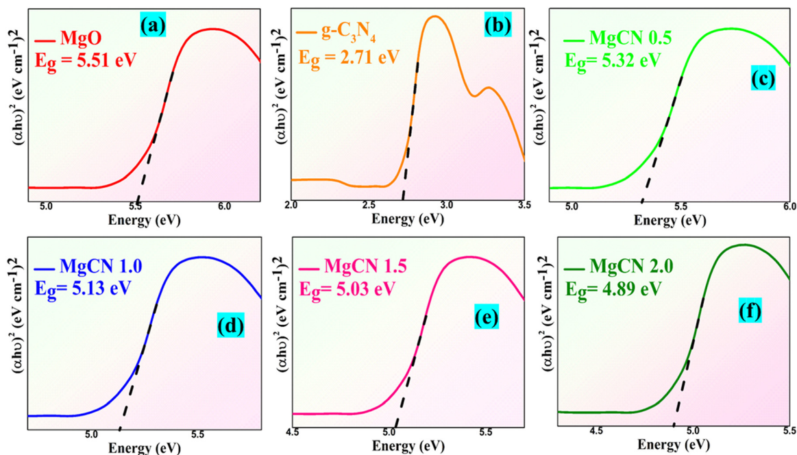
Fig. 11 UV-Vis assisted bandgaps of the MgO (a), g-C_3N_4 (b), and MgCN nanocomposite at 0.5, 1.0, 1.5, and 2.0 mM (c)–(f), respectively.
