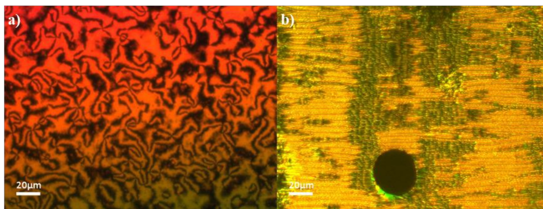
Figure 5. Textures observed for CBS6CT: (a) schlieren texture of the nematic phase ( T = 157^{\circ}\text{C} ) and (b) rope-like textures coexisting with a polygonal texture of the twist-bend nematic phase ( T = 95^{\circ}\text{C} ).
