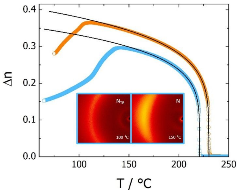
Figure 6. Temperature dependence of the optical birefringence for CBS9OCT (orange circles) and CBS10CT (blue squares) measured with green light ( \lambda = 532 nm) on cooling. Black lines show fitted power-law dependencies. Inset: 2D X-ray diffraction patterns for CBS9OCT in the: (right) N phase ( T = 150^\circ\text{C} ) and (left) N_{TB} phase ( T = 100^\circ\text{C} ).
