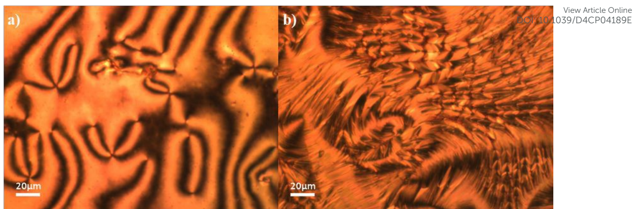
Figure 4. Textures observed for CBS7OCT; (a) schlieren texture of the nematic phase ( T = 205\text{ }^{\circ}\text{C} ) and (b) focal conic regions with blocky schlieren texture of the twist-bend nematic phase ( T = 111\text{ }^{\circ}\text{C} ).
