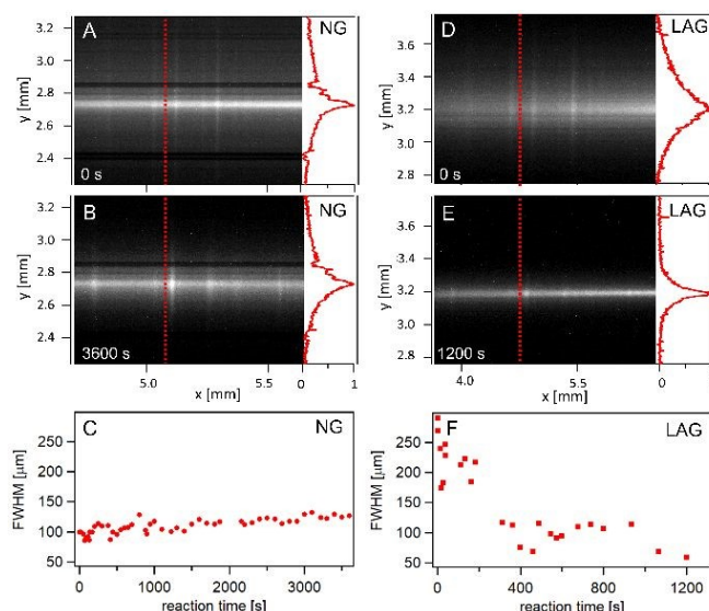
Figure 7. Monitoring of sample rheology under NG (A, B, and C) and LAG conditions (D, E, and F) during the reaction between ZnO and HIm. Spectra are shown at the beginning (0 s) and the end of the reaction (3600 s for NG, 1200 s for LAG). The normalized intensity profile along 1300\text{ cm}^{-1} (fluorescence signal only, red dashed line) is displayed at the right edge of each spectrometer image section (red line, referred to as the y -axis signal in the text). Panels C and F illustrate the evolution of the FWHM of the y -axis signal throughout the NG and LAG reactions, respectively. The dark horizontal stripes in A and B result from dust particles adhered to the entrance slit.
