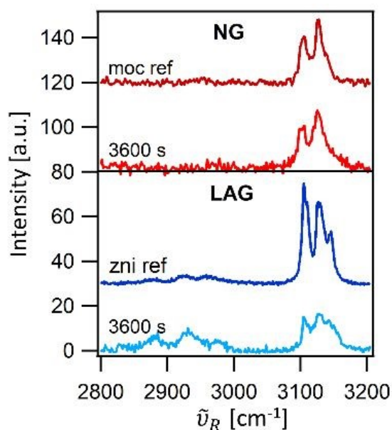
Figure 6. Raman spectra in high-frequency region of the moc product (dark red and red line) and of the zni product (blue and light blue line): taken ex situ with a commercial research grade Raman system ( moc ref and zni ref) and in situ with our mechanochemical Raman system at the end of the NG and the LAG reactions (3600 s red and blue, respectively).
