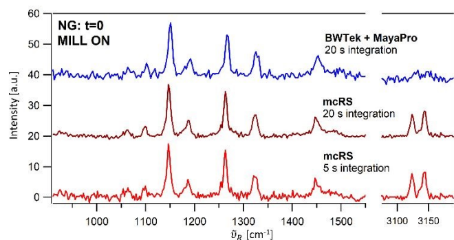
Figure 3. Comparison of the Raman spectra collected at beginning of milling of imidazole with the standard fiber-optics Raman system using 20 s integration (blue), and with mcRS using 20 s integration (dark red) and 5 s integration (red). Power of the excitation source: 300 mW for fiber-optics spectrometer and 25 mW for mcRS.
