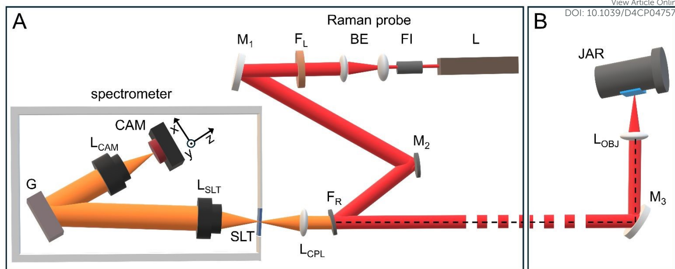
Figure 1. A. Scheme of the mechanochemistry Raman System (mcRS), top view: laser L, Faraday isolator FI, beam expander BE, laser filter F_L , Raman edge filter F_R , coupling lens L_{CPL} , entrance slit SLT, slit lens L_{SLT} , diffraction grating G, camera lens L_{CAM} , iCMOS camera CAM. Dashed red line depicts the laser beam that continues up to M_3 ; B. Side view of the setup in the vicinity of the jar with the vertical folding mirror M_3 , the objective lens L_{OBJ} and the aluminium jar with sapphire window (blue rectangle).
