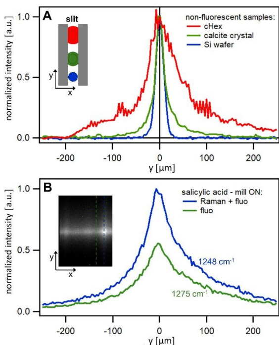
Figure 2. A. The Raman signal profile taken along the y -axis for a Si wafer (blue), a 0.3 mm thick calcite crystal (green) and cyclohexane liquid (red). The inset illustrates how the excitation footprint increases with penetration depth of the laser and gets imaged on the entrance slit. B. The Raman signal profiles taken along the y -axis for a salicylic acid sample during milling. The blue line is the signal at a Raman peak, while the green line is a pure fluorescence signal. The inset shows an image taken with the iCMOS camera, the dashed lines show where the y -axis profiles were taken.
