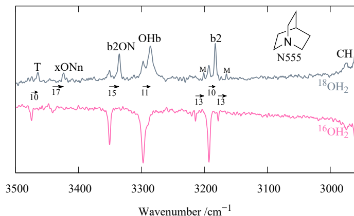
Fig. 5 Comparison of the OH stretching spectrum of N555 with ^{16}\text{OH}_2 (bottom, inverted) to the same spectrum enriched in ^{18}\text{OH}_2 . The 16-18-isotope shifts in \text{cm}^{-1} are clarified by arrows (see Table S15 in the ESI† for details).
