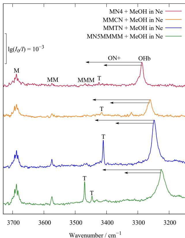
Fig. 11 Spectra for methanol complexes of four tertiary amines, with strong OHb stretching signals from monohydrates besides dihydrates (T) and methanol (M) homodimers (MM) and -trimers (MMM). Arrows indicate where bands with OHbON character would be expected in an (ON unscaled) harmonic DFT picture (two monohydrate vibrations carry significant ON stretching character).
