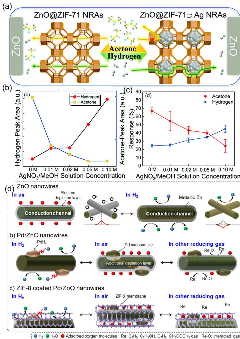
Fig. 14 (a) Schematic illustration of \text{H}_2 sensing by tuning the molecular sieving properties of ZIF-71 by incorporating Ag NPs. (b) The total desorption peak area control of acetone-TPD spectra and \text{H}_2 -TPD spectra. (c) The sensing response of \text{ZnO@ZIF-71-Ag} NRAs for various Ag NPs concentration loading to 20 ppm \text{H}_2 and acetone. Reproduced with permission from ref. 226 Copyright 2021, Royal Society of Chemistry. (d) Schematic illustration of the sensing mechanism for ZnO NWs, Pd/ZnO NWs and ZIF-8/Pd/ZnO NWs. Reproduced with permission from ref. 227 Copyright 2018, American Chemical Society.
