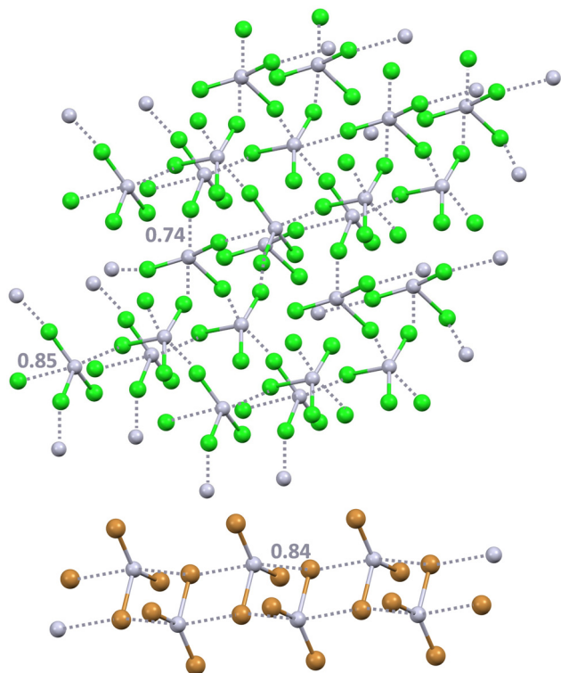
Fig. 16 Ball and stick representation of the supramolecular anionic 3D network formed by \text{HgCl}_3^- via SpBs in the methylammonium salts (Refcode QQQBVL04) 170 (top) and the 1D network formed by \text{HgBr}_3^- in the salt with a benzimidazolium derivative (Refcode WURPOP) 171 (bottom). Cations have been omitted for clarity; SpBs are shown in grey dotted lines. Nc values of SpBs are reported close to the interactions. Colour code: light grey, mercury; green, chlorine; and ochre, bromine.
