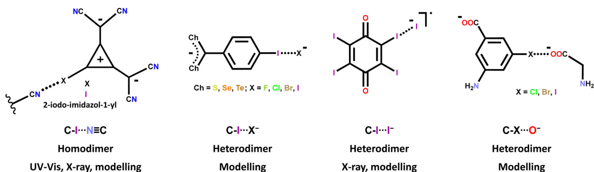
Scheme 4 Structural formulas of some halocarbons forming halogen bonded anion \cdots anion adducts. The interaction and adduct features and the used analytical techniques are also given.
