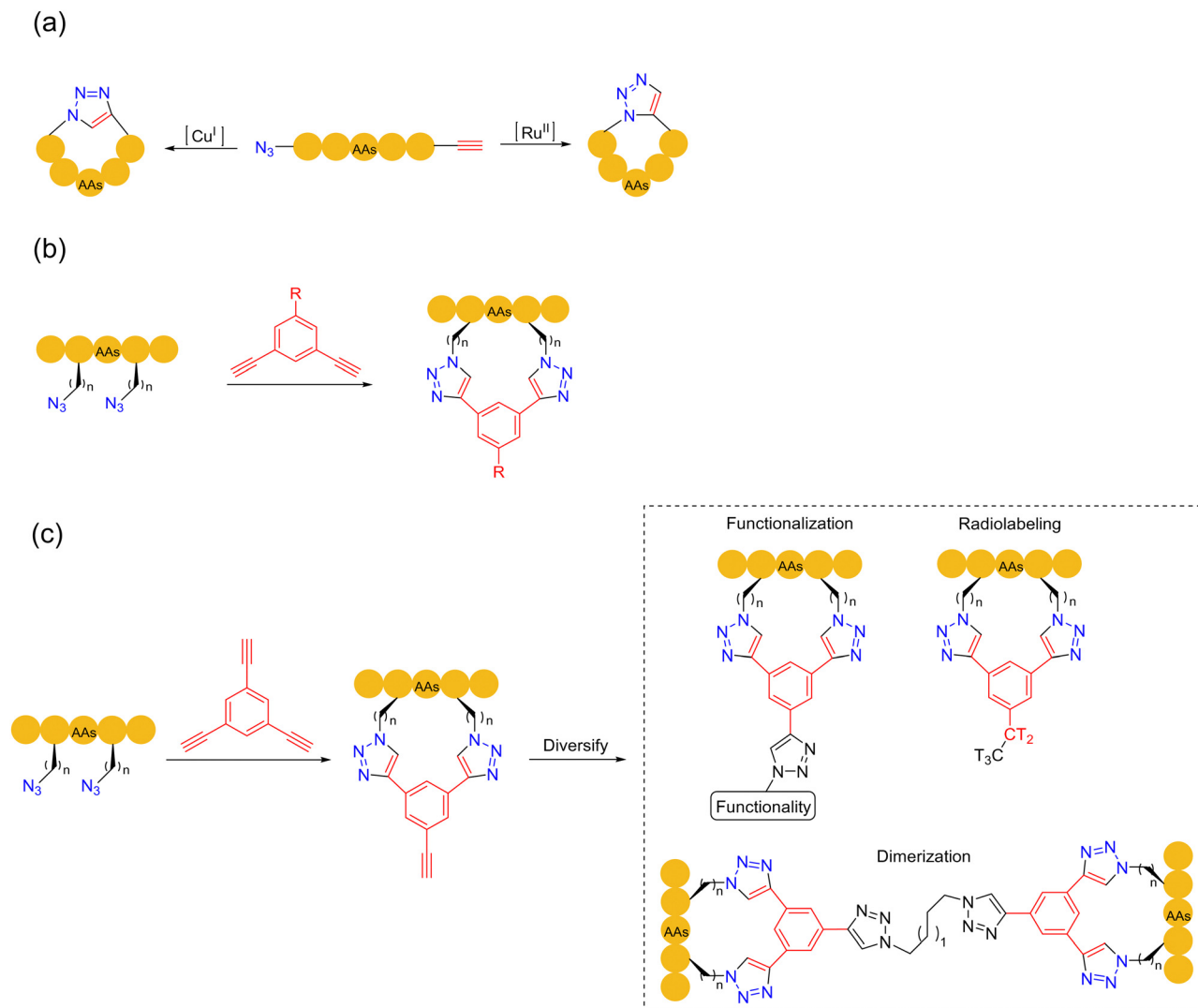
Scheme 15 Azide-alkyne click cycloaddition-based peptide macrocyclization strategies. (a) CuAAC and RuAAC; (b) and (c) click-stapling.
