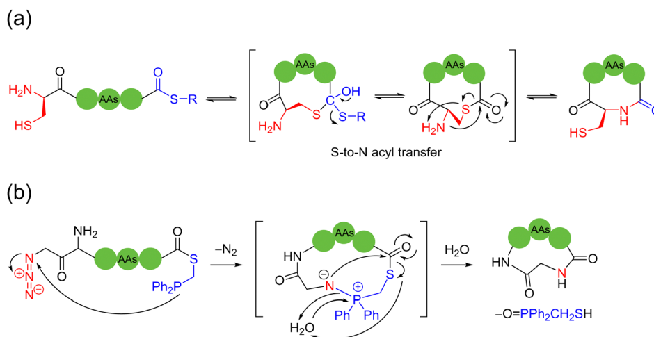
Scheme 1 Selected representative ligation-mediated peptide macrocyclization strategies. (a) 1,2-Aminothiols and thioester ligation and S -to- N acyl transfer (native chemical ligation, NCL) and (b) azide and phosphine-linked thioester Staudinger ligation.
