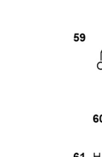
Fig. 12 Kinetically stable organic cages can be prepared via a variety of methodologies and using myriad reactions. R groups omitted from SCXR structures for clarity.
