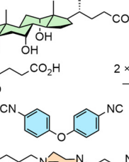
Fig. 12 Kinetically stable organic cages can be prepared via a variety of methodologies and using myriad reactions. R groups omitted from SCXR structures for clarity.
