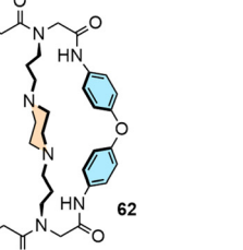
Fig. 12 Kinetically stable organic cages can be prepared via a variety of methodologies and using myriad reactions. R groups omitted from SCXR structures for clarity.
