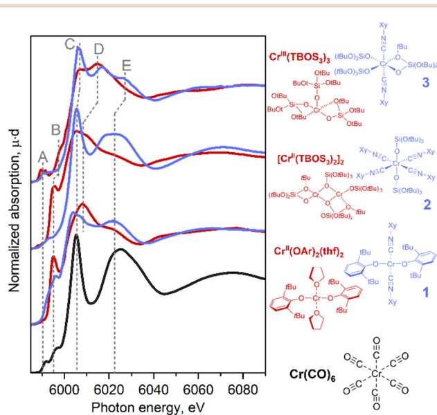
Fig. 1 Experimental Cr K-edge XANES spectra for \text{Cr}(\text{CO})_6 (black) and the series of isocyanide complexes (blue) compared with similar reference complexes without isocyanide ligands (red).
