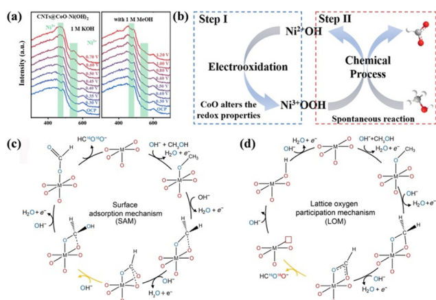
Fig. 2 (a) In situ Raman spectra of the OER and MOR for \text{CNTs@CoO-Ni(OH)}_2 . (b) Dynamic reconstruction of the active \text{Ni}^{3+}\text{OOH} layer. 56 Reproduced from ref. 56 with permission from the Royal Society of Chemistry, Copyright 2023. Possible reaction mechanisms for (c) SAM and (d) LOM. 63 Reproduced from ref. 63 with permission from American Association for the Advancement of Science, Copyright 2023.
