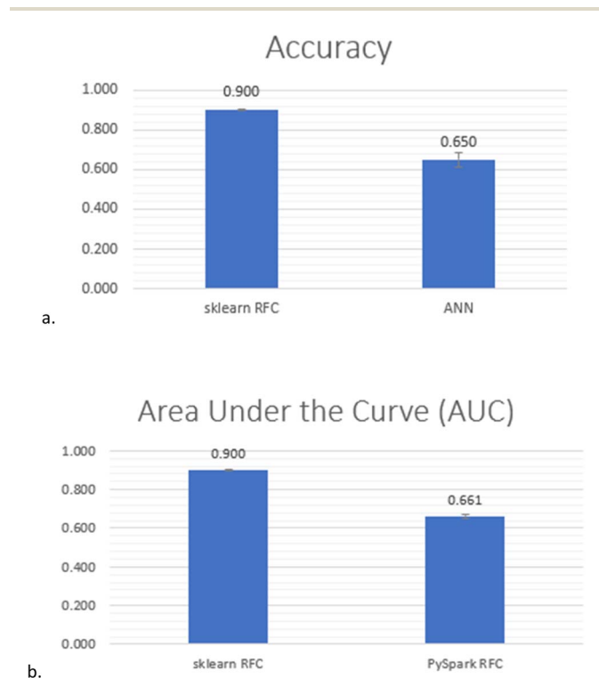
Fig. 5 Final comparison between PySpark RFC, scikit RFC and ANN, (a) scikit RFC vs. ANN tuned with Optuna and (b) Scikit RFC vs. PySpark RFC.
