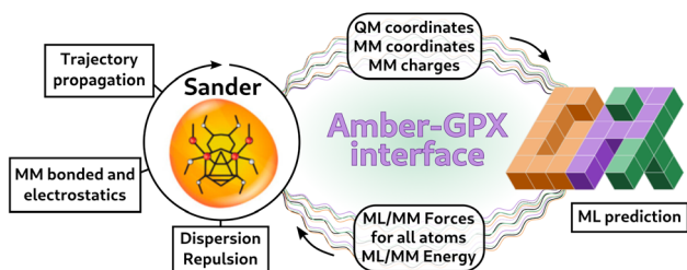
Fig. 3 Scheme representing the Amber-GPX interface via the ML-server program. 52 At each step of the dynamics, Sander computes the MM energies and forces, and the ML-MM dispersion and repulsion interaction. Coordinates and charges are sent to the Python server, and are used by GPX models to predict the energies and forces of the ML part, as well as the MM forces coming from the ML-MM interaction. This information is sent back to Sander, which performs one step of the trajectory.
