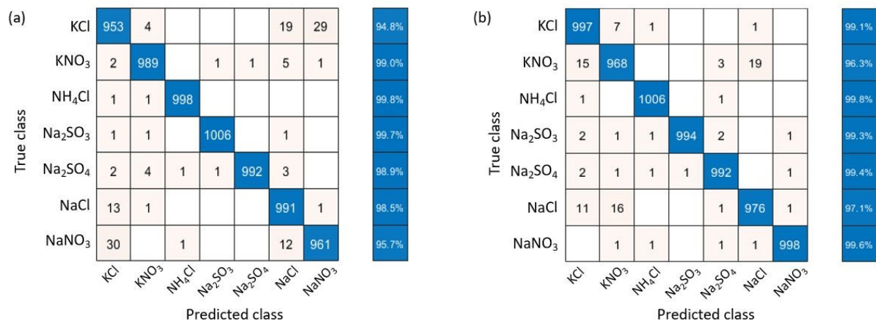
Fig. 7. Confusion matrices for identifying the salt type regardless of concentration. The results follow from the ML classifier (a) “Random Forest” with 100 decision trees and (b) XGBoost. Both sets of results are based on 20 repeats with different random number seeds. We used 70% of the 23,417 sample entries for training and 30% ( N = 7025 ) for testing. The numbers in the matrix cells denote the averages per run and the right column shows the correct predictions per salt. As obtained from the mean and standard deviation of the repeated runs, the overall accuracy is (a) (98.1 \pm 0.1)\% and (b) (98.6 \pm 0.1)\% .
