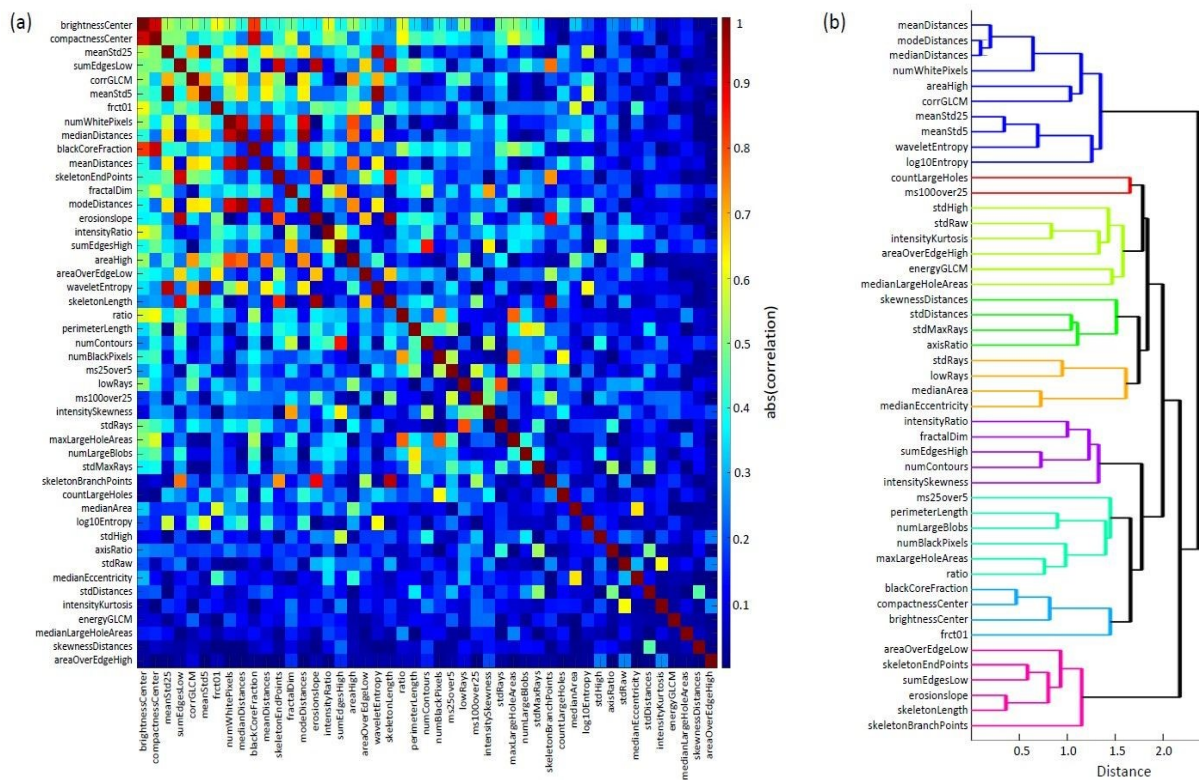
Fig. 5. Correlation analysis of the metrics based on the Z-scored data. (a) Heatmap of the reordered absolute correlation coefficient matrix. The color scale represents the absolute value of the correlation coefficients. Metrics are sorted according to their average absolute correlations with the other metrics. Metrics listed near the bottom stand out as having little similarity to the other metrics. (b) Alternative grouping of the metrics using hierarchical clustering. The dendrogram shows relationships and groupings of the metrics. The x-axis represents the Euclidean distance calculated from the absolute correlation values, where shorter distances indicate stronger relationships and higher similarity between metrics.
