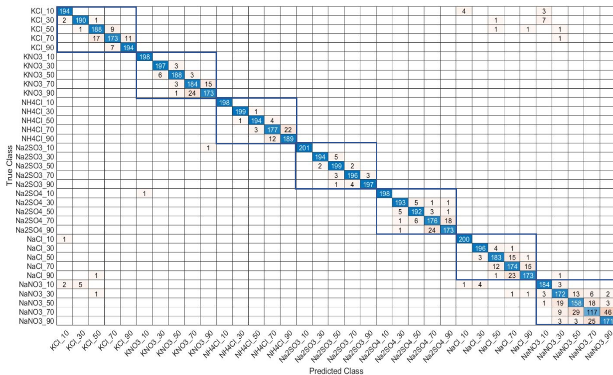
Fig. 8. Confusion matrix for identifying the salt type and the initial concentration. The results are obtained from deep learning using a Multi-Layer Perceptron (MLP) architecture. We used 70% ( N = 16392 ) of the 23,417 sample entries for training and 30% ( N = 7025 ) for testing. The confusion matrix presented here represents the average results over 20 runs. The numbers in the matrix cells denote the average occurrences per run. As determined by the mean and standard deviation across the repeated runs, the overall accuracy of the model is (92.5 \pm 0.4)\% .
