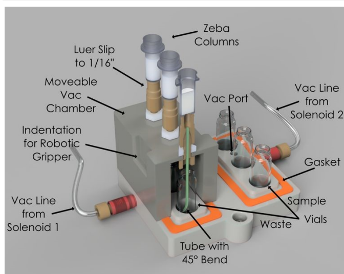
Fig. 5 Schematic of the custom vacuum filtration module for automated antibody purification. The system integrates Zeba spin columns into a moveable vacuum chamber, controlled via solenoid-actuated vacuum lines for precise filtration.
