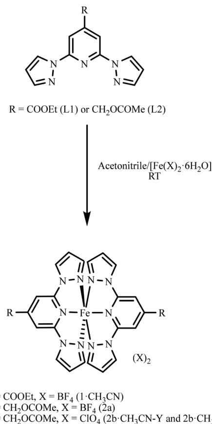
Scheme 1 Preparation of complex 1 -CH 3 CN from L1 and complexes 2a and 2b -CH 3 CN from L2 . Two different polymorphs coloured yellow ( 2b -CH 3 CN- Y ) and red ( 2b -CH 3 CN- R ) were obtained for 2b -CH 3 CN.
