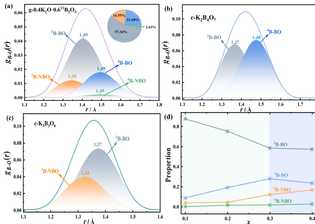
Fig. 4 (a), (b) and (c) represent the distribution of {}^3\text{B-O} , {}^3\text{B-NBO} , {}^4\text{B-O} and {}^4\text{B-NBO} interactions in the first coordination layer of the B–O interaction in 0.40\text{K}_2\text{O}\cdot 0.60{}^{11}\text{B}_2\text{O}_3 glass and \text{K}_2\text{B}_4\text{O}_7 and \text{K}_3\text{B}_3\text{O}_6 crystals, respectively. The inset pie chart in the panel for 0.40\text{K}_2\text{O}\cdot 0.60{}^{11}\text{B}_2\text{O}_3 glass shows the percentages of each atom-pair interaction. (d). The relative contents of the {}^3\text{B-O} , {}^3\text{B-NBO} , {}^4\text{B-O} and {}^4\text{B-NBO} interactions in x\text{K}_2\text{O}\cdot (1-x){}^{11}\text{B}_2\text{O}_3 ( 0.1 \leq x \leq 0.4 ) glass.
