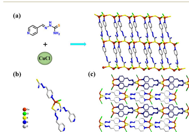
Fig. 1 (a) The constituents and two-dimensional lamellar structure of CuCl-Pyhc. (b) Connecting configuration between the ligands and the Cu atom. (c) Stacking in an ABAB fashion of CuCl-Pyhc.
