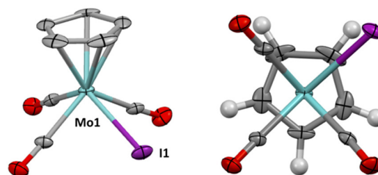
Fig. 8 Molecular structure of [MoI(CO) _3 ( \eta^5 -C _5 H _5 )] in a crystal (50% displacement ellipsoids, most hydrogen atoms omitted).
