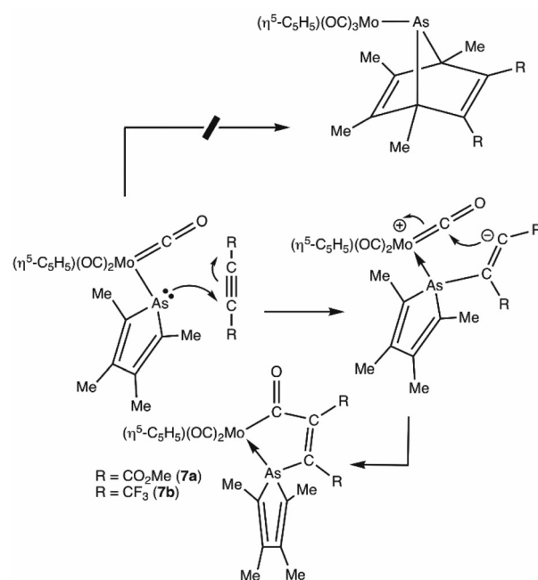
Scheme 5 [3 + 2] -cycloaddition of a \sigma -arsolyl complex 1a with activated alkynes (R = \text{CF}_3 , \text{CO}_2\text{Me} ).
