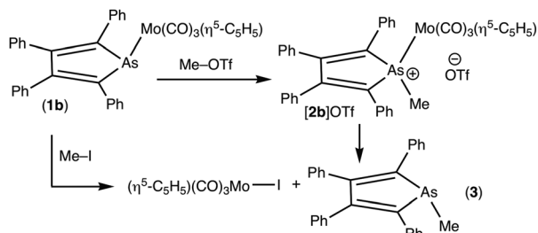
Scheme 3 Attempted methylation of a tetraphenylarsolyl complex.
