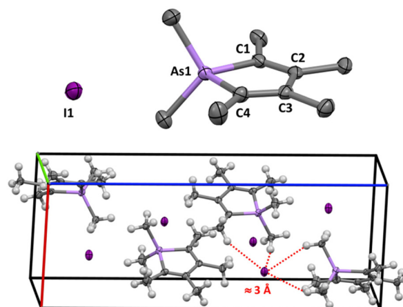
Fig. 6 The molecular structure of [4]I in a crystal (50% displacement ellipsoids, methyl groups simplified and hydrogen atoms omitted). Inset: The unit cell contents ( P2_1/c ) viewed along the crystallographic b axis highlighting extended \text{H}\cdots\text{I}^- interactions.
