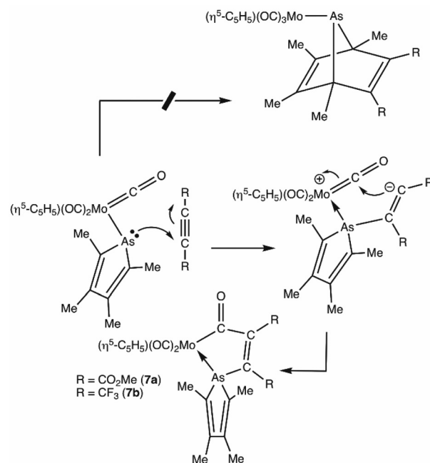
Scheme 5 [3 + 2] -cycloaddition of a \sigma -arsolyl complex 1a with activated alkynes ( \text{R} = \text{CF}_3, \text{CO}_2\text{Me} ).
