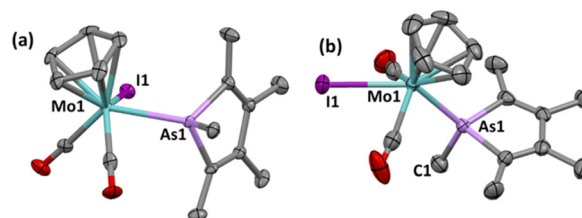
Fig. 9 Isomeric pentamethylarsole complexes. Molecular structures of (a) cisoid -[MoI(MeAsC _4 Me _4 )(CO) _2 ( \eta^5 -C _5 H _5 )] ( cisoid -5) in a crystal (one of two crystallographically unique molecules) and (b) transoid -[MoI(MeAsC _4 Me _4 )(CO) _2 ( \eta^5 -C _5 H _5 )] ( transoid -5) in a co-crystallite of ( transoid -5) _{0.11} (6) _{0.89} . (50% displacement ellipsoids, methyl groups simplified and most hydrogen atoms omitted).
