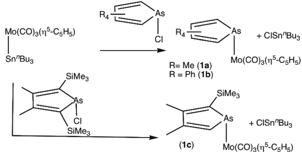
Scheme 1 Synthesis of \sigma -arsolyl complexes via transmetalation. 2c
