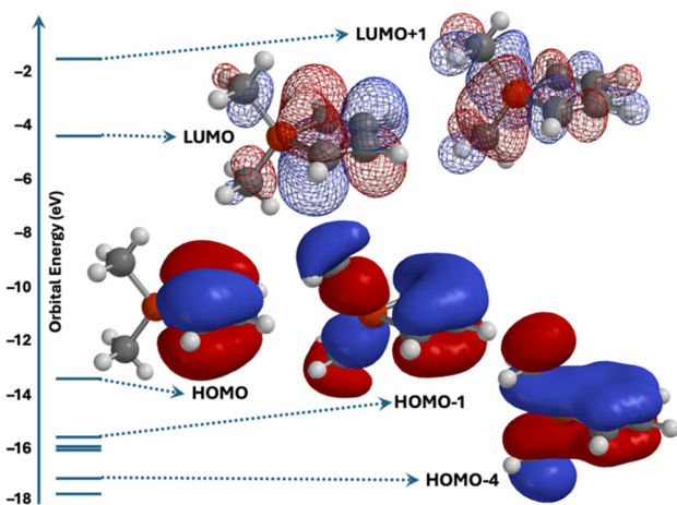
Fig. 7 Frontier orbitals of interest for the hypothetical dimethyl-arsolylum cation [Me _2 AsC _4 H _4 ] ^+ (DFT: \omega B97X-D/6-31G*/gas phase).
