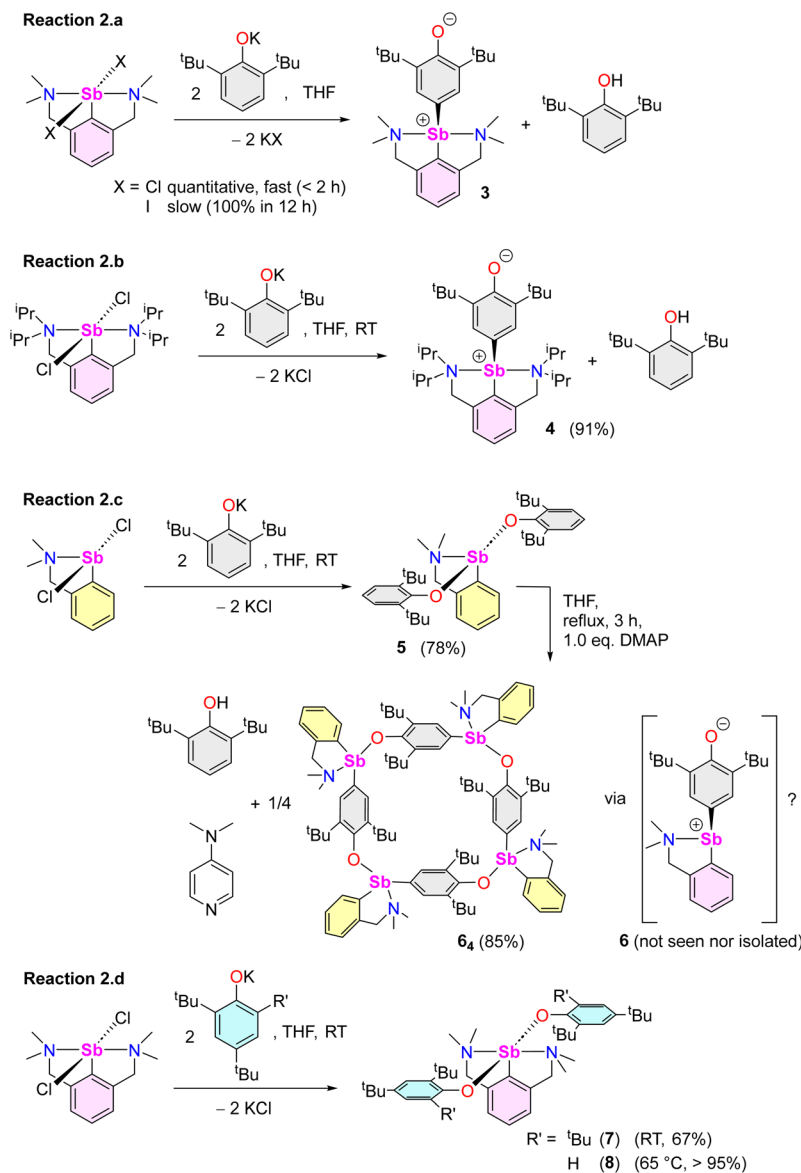
Scheme 2 Reactions of Sb(III) dihalides with potassium phenolates.
