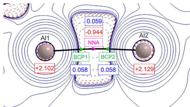
Fig. 3 Laplacian operator of the electron density in a plane containing both Al nuclei of [(DNI(H)Al)_2] ( 2 ). Contours are drawn in a logarithmic scale: positive as solid blue lines and negative ones as dashed red lines. The non-nuclear attractor (NNA) is depicted in a magenta box, bond critical points (BPCs) are given in green box, and AIM charges are given in red boxes for both Al ions and charge density magnitude at both bond critical points and the NNA are given in blue boxes ( \text{e}^- \text{ Bohr}^{-3} ).
