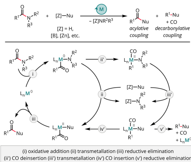
Scheme 7 General 2e^- redox-cycling mechanism proposed for acylative and decarbonylative coupling reactions with \text{C}(\text{acyl})\text{--N} electrophiles. Nu = nucleophile.
