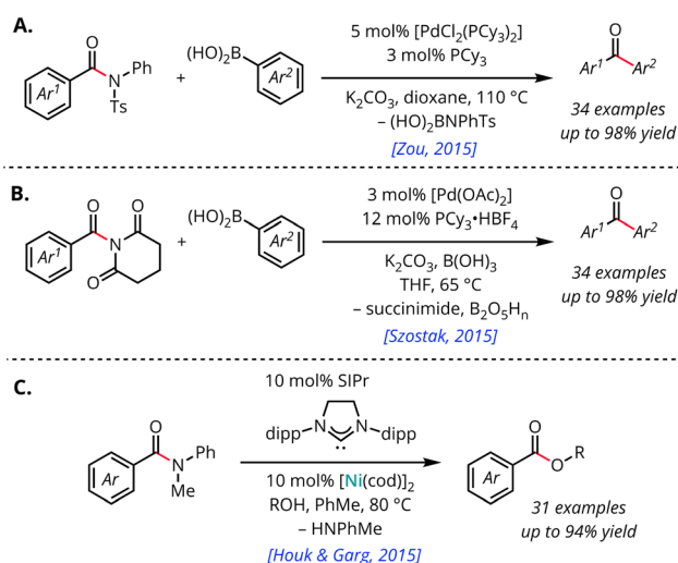
Scheme 8 Key early developments in Pd- and Ni-catalysed acylative coupling using \text{C}(\text{acyl})\text{--N} electrophiles. Ar = aryl; cod = 1,5-cyclooctadiene; dipp = 2,6-diisopropylphenyl; Ts = 4-toluenesulfonyl.
