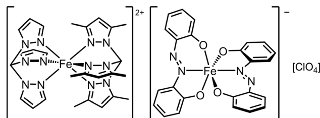
Scheme 5 The [\text{Fe}^{\text{II}}(\text{tpm})(\text{tpm}')][\text{Fe}^{\text{III}}(\text{azp})_2][\text{ClO}_4]_2 SCO double salt. 130
