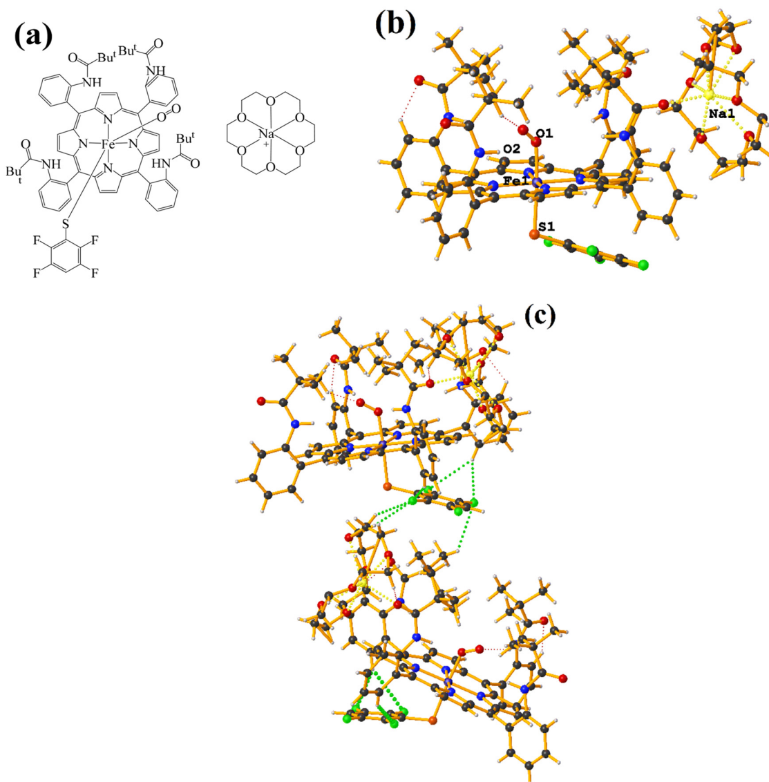
Fig. 19 (a) Schematization of the molecular structure GAHQLOQ. (b) Molecular structure of GAHQLOQ. For clarity, the numbering of the atoms is not shown. (c) Supramolecular array of GAHQLOQ.
