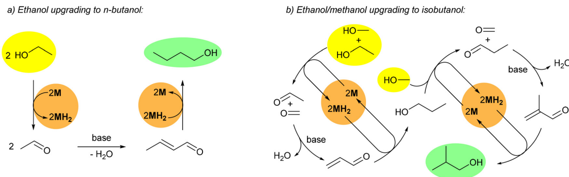
Scheme 1 Production of n -butanol and isobutanol using Guerbet chemistry. \text{MH}_2 can be a conventional metal dihydride or involve metal–ligand cooperativity.
