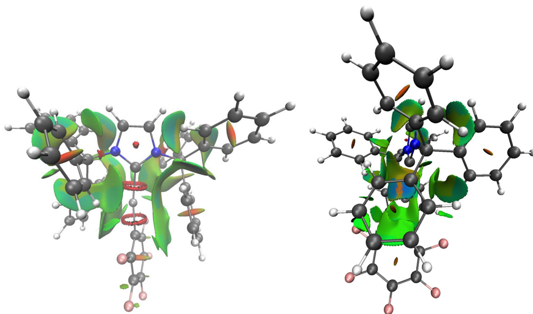
Fig. 5 Non covalent interactions (NCI) isosurface ( h = 0.65 ) for model cation [(ITr)Zn(C_6F_5)]^+ (VI), as estimated by DFT calculations at the \omega B97XD/6-31+G** theory level. Green areas correspond to attractive van der Waals interactions, blue areas indicate electrostatic interactions, and red areas indicate repulsive steric congestion.
