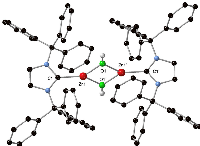
Fig. 6 Molecular structure of Zn dication [(\text{ITr})\text{Zn}(\mu\text{-OH})_2]^{2+} ( [\mathbf{11}]^{2+} ). Selected bond distances (Å) and angles (°). \text{Zn1-C1} = 1.980(2) , \text{C1-N1} = 1.361(3) , \text{C1-N2} = 1.356(3) , \text{Zn1-O1} = 1.907(2) , \text{Zn1'-O1} = 1.938(2) , \text{O1-Zn1-C1} = 146.30(8) , \text{O1-Zn1-O1'} = 80.16(8) , \text{Zn1-O1-Zn1'} = 99.84(8) .
