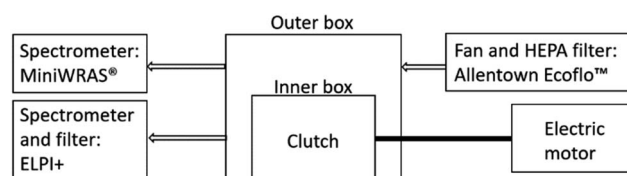
Fig. 2 Schematic depiction of the experimental setup.
