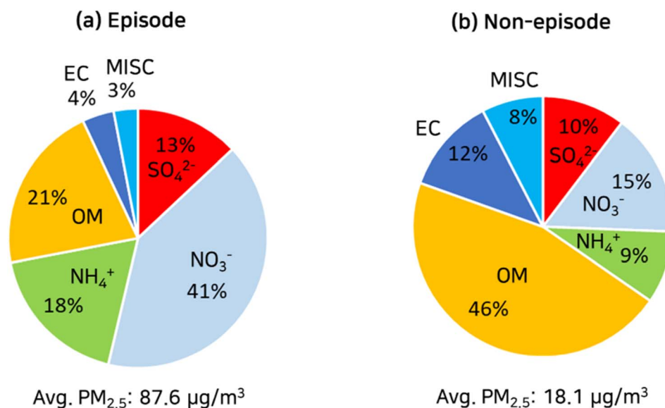
Fig. 3 Mass fractions of PM_{2.5} chemical compositions measured at the SU supersite during the episode (a) and non-episode (b) in January 2018.
