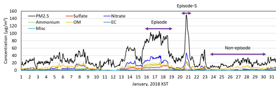
Fig. 2 PM_{2.5} mass and particulate species concentrations measured at the SU supersite in January 2018.
