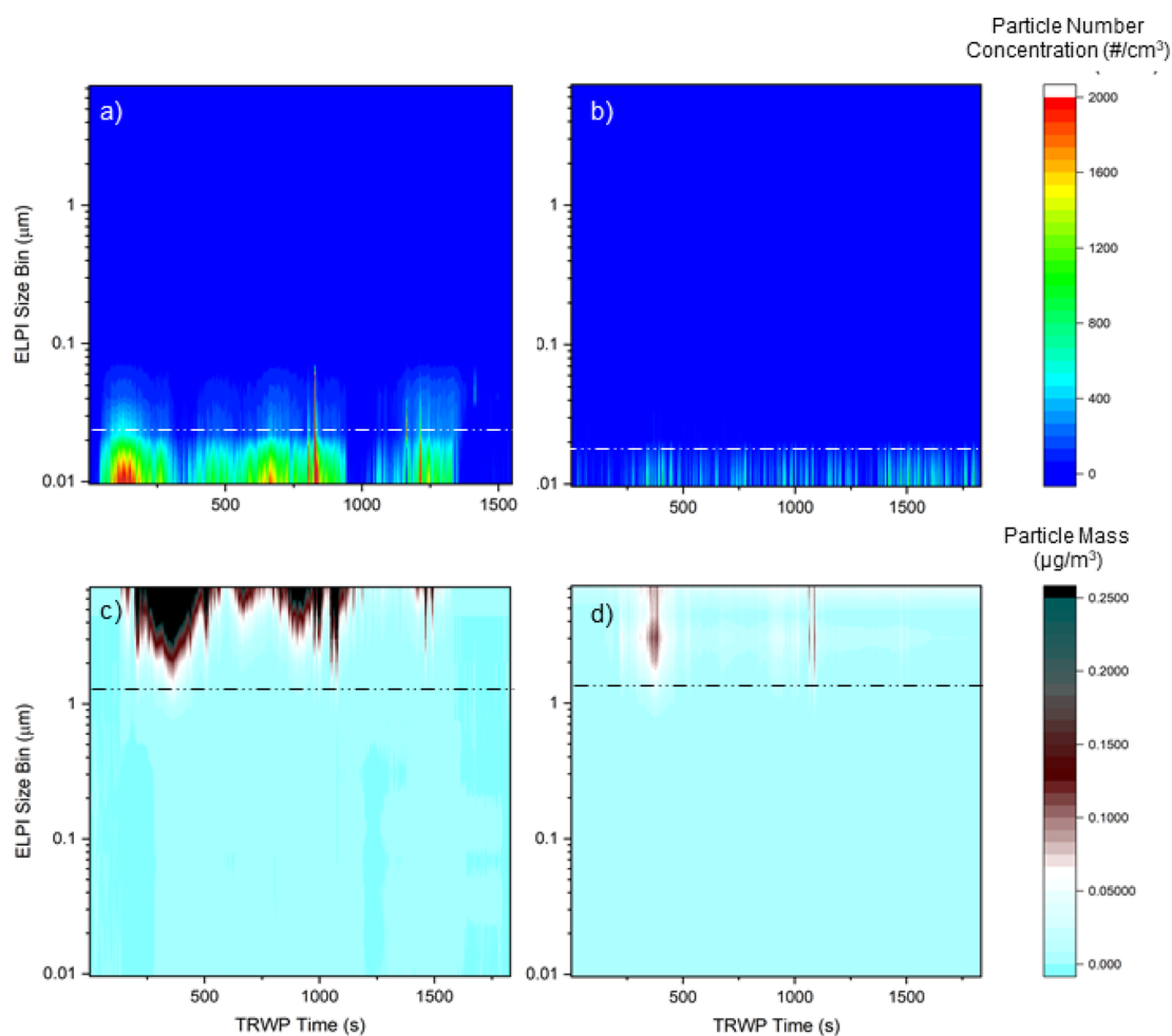
Fig. 4 The size distribution is shown for the entire drive cycle driven displayed by particle number concentration for data (a) without the CS (total particle number) and (b) with the CS (solid particle number) in comparison to the mass distribution by size bins for data (c) without the CS data (total particle mass) and (d) with the CS (solid particle mass). Data below the dashed line (a and b) represent the size bins where 95% of the particle number concentration is collected and data in size bins above the black dashed line (c and d) comprise 95% of the mass concentration. These data are background corrected.
