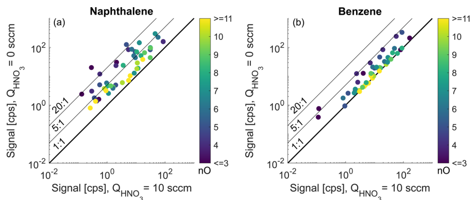
Fig. 5 Comparison of sensitivity enhancement for oxidation products as a response to a decrease in the HNO 3 concentration in the CI-inlet in the high RO 2 regime between naphthalene (a) and benzene experiments (b) (exp. 2 and 4). The enhancement ratio is the slope on this figure, and color is the number of oxygen atoms ( n_{\text{O}} ).
