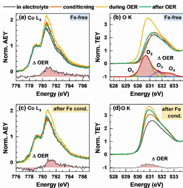
Fig. 5 In situ near-edge X-ray absorption fine structure (NEXAFS) measurements of Co 3 O 4 NPs during the OER before (a) and (b) and after (c) and (d) conditioning with 5 ppm Fe. Measurements were performed in 0.1 M KOH with 5 ppm Fe at 1 V RHE , after the conditioning at 1 V RHE , during the OER at 1.6 V RHE with exchanged, Fe free 0.1 M KOH and after the OER at 1 V RHE . (a) and (c) In situ Co L-edge Auger electron yield (AEY) spectroscopy ( E_{\text{kin}} = 656 eV) normalized by the intensity at 778.5 eV with the differential spectrum OER – after the OER. (b) and (d) In situ total electron yield (TEY) O K spectrum normalized on the intensity at 534 eV of the O K background signal from the membrane and water signal. The differential spectrum OER – after the OER for the Fe-free measurements was fitted with a Gaussian distribution function and shows 4 different oxygen species O 1 –O 4 created during the formation of electrophilic oxygen.
