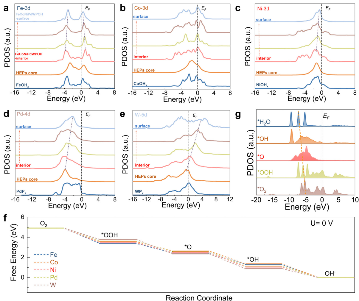
Fig. 6 DFT calculations for ORR. (a)–(e) Site-dependent PDOSs of Fe, Co, Ni, Pd, and W sites in the FeCoNiPdWPOH structure. (f) Standard free energy diagram of the ORR process at 0 V of various active sites on the surface-reconstructed samples. (g) PDOS of key intermediates over Pd sites in FeCoNiPdWPOH.
