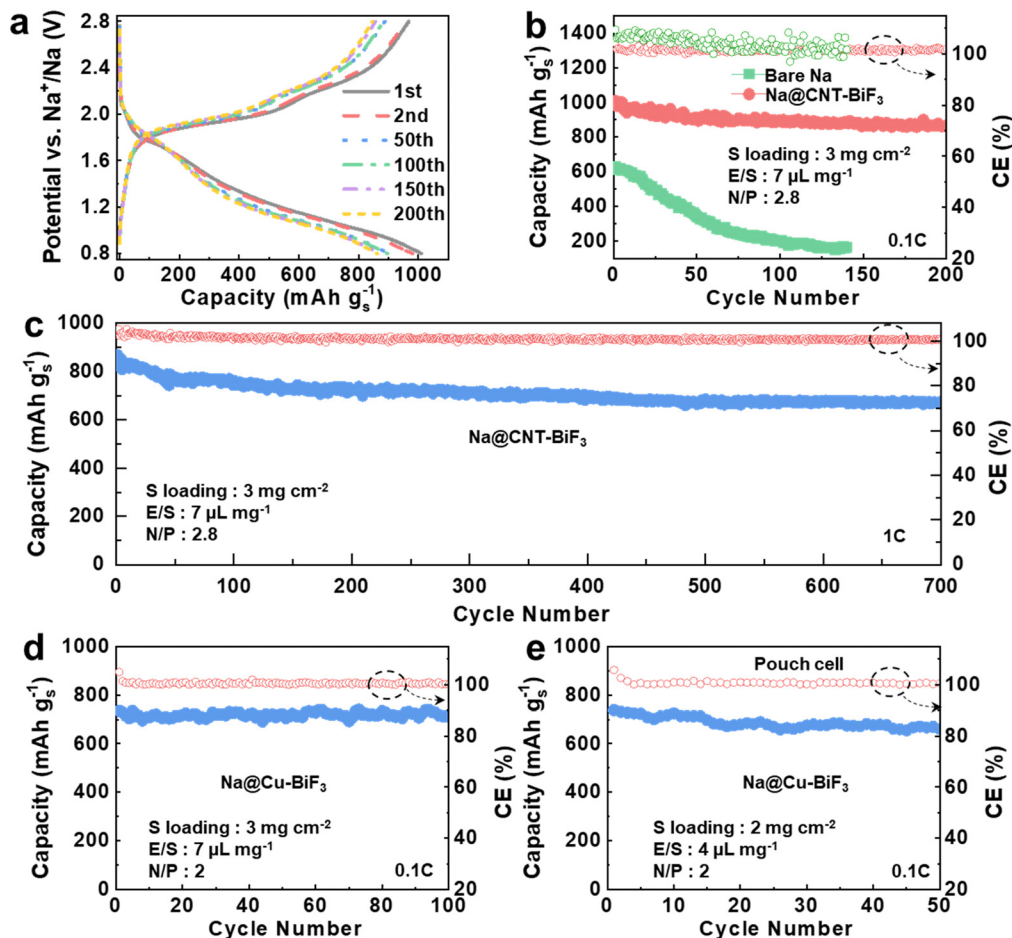
Fig. 7 Electrochemical performance of Na@CNT-BiF 3 and Na@Cu-BiF 3 . (a) Voltage profiles of Na@CNT-BiF 3 at various cycles. (b) Cycling performances of bare Na and Na@CNT-BiF 3 electrodes at 0.1C rate. (c) Cycling performance of Na@CNT-BiF 3 electrodes at 1C rate. Cycling performances of Na@Cu-BiF 3 electrodes in (d) coin cell and (e) pouch cell at 0.1C rate.
